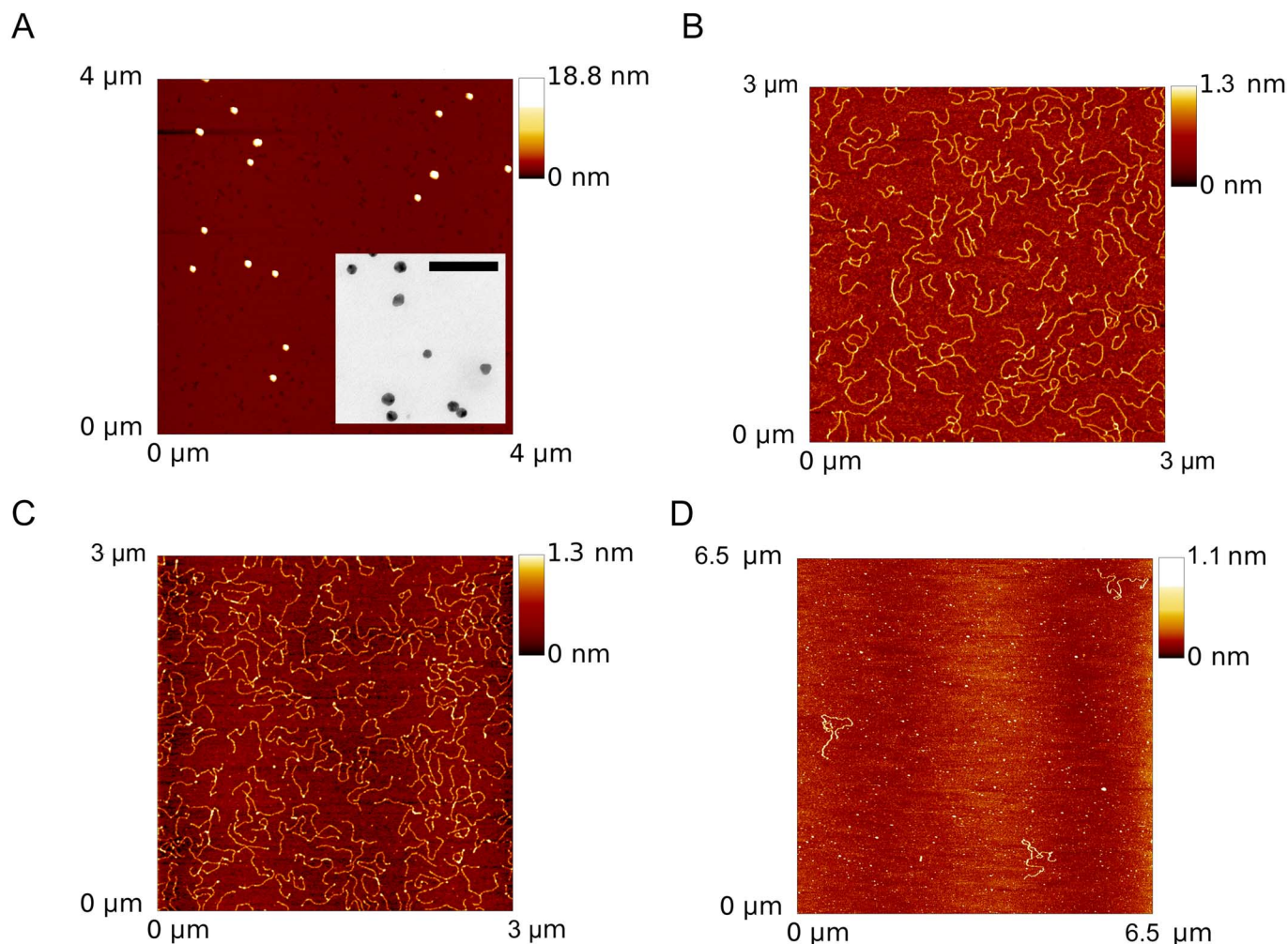
Fig 2. AFM images of: (A) the Au nanoprobes alone—inset shows TEM of bare gold clusters, scale bar = 100 nm); and (B) DNA alone, namely the 1559 bp complementary PCR product; (C) the 1565 bp noncomplementary PCR product; and (D) the \approx 8668 bp linearized p158 plasmid.
