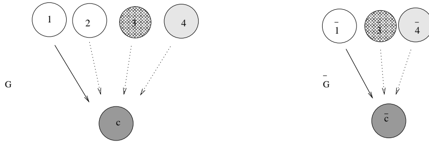
Figure 8: A coupled cell graph G and the corresponding natural quotient graph \bar{G} given by the equivalence relation \bowtie with classes \{1, 2\} , \{3\} , \{4\} and \{c\} .
