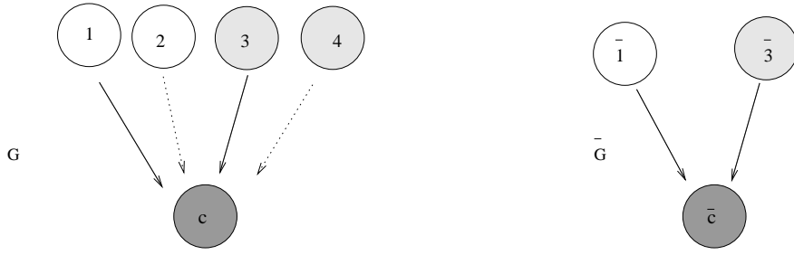
Figure 10: A coupled cell graph G and the corresponding natural quotient graph \bar{G} given by the equivalence relation \bowtie with classes \{1, 2\} , \{3, 4\} and \{c\} .
