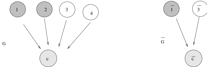
Figure 4: A coupled cell graph G and the corresponding quotient graph \overline{G} given by the \bowtie -equivalence relation with classes \{1, 2\} , \{3, 4\} and \{c\} .
