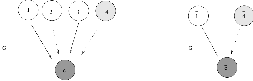
Figure 6: A coupled cell graph G and the corresponding natural quotient graph \bar{G} given by the equivalence relation \bowtie with classes \{1, 2, 3\} , \{4\} and \{c\} .
