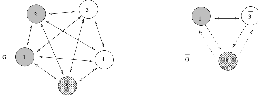
Figure 9: A coupled cell graph G with \mathbf{S}_5 -symmetry and the corresponding natural quotient graph \overline{G} with \mathbf{Z}_2 -symmetry given by the equivalence relation \bowtie with classes \{1, 2\} , \{3, 4\} and \{5\} .
