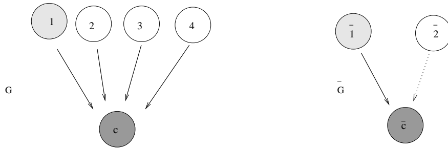
Figure 5: A coupled cell graph G and the corresponding natural quotient graph \overline{G} given by the equivalence relation \bowtie with classes \{1\} , \{2, 3, 4\} and \{c\} .
