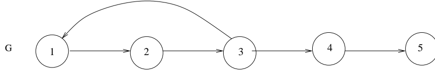
Figure 1: An example of a coupled cell graph G .
