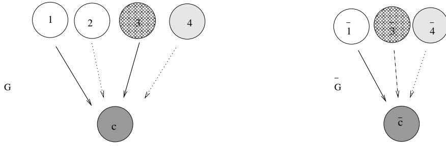
Figure 7: A coupled cell graph G and the corresponding natural quotient graph \bar{G} given by the equivalence relation \bowtie with classes \{1, 2\} , \{3\} , \{4\} and \{c\} .
