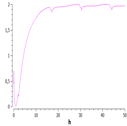
Figure 8.2: Cyclin D with inefficient Ras-GTP hydrolysis
