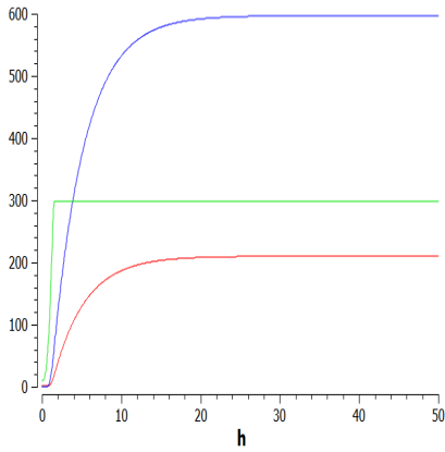
Figure 8.1: ERG (blue), DRG (red) and ERK-PP (green) with inefficient Ras-GTP hydrolysis, Raf dephosphorylation or dephosphorylation of ERK-P
