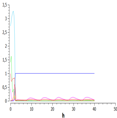
Figure 8.5: Cyclins, CDH1 (dark blue) and CDC20 (red) regulation with strong dependency on and fast production of GAP
