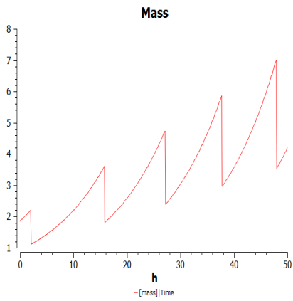
Figure 10.3: Mass in estrogen-dependent cell model
