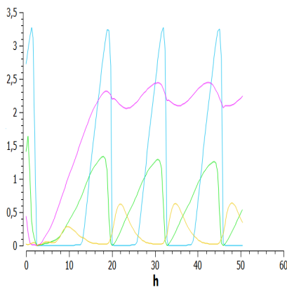
Figure 11.3: Cyclins concentration in hyperactive-Ras cell treated with ERK inhibition.
