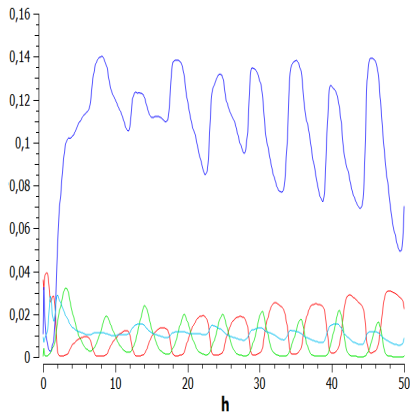
Figure 8.12: p27:CycD:CDK4 (dark blue) and all other forms of p27 in CDH1 -deficient cell
