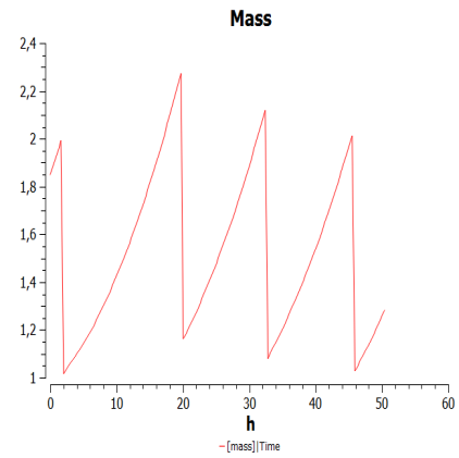
Figure 11.6: Mass of the cell with hyperactive-Ras treated with ERK inhibition.
