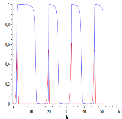
Figure 11.4: CDH1 and CDC20 in hyperactive-Ras cell treated with ERK inhibition.
