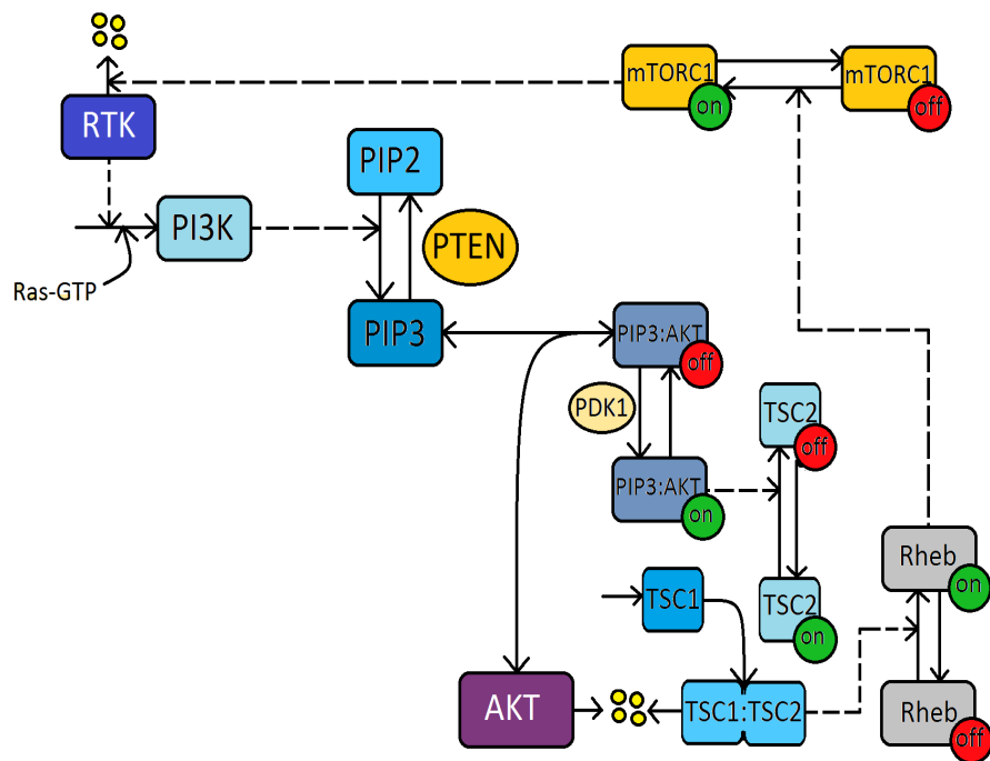
Figure 4.2: The PI3K/AKT signalling pathway
