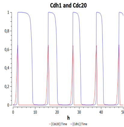
Figure 10.2: CDH1 and CDC20 in estrogen-dependent cell model
