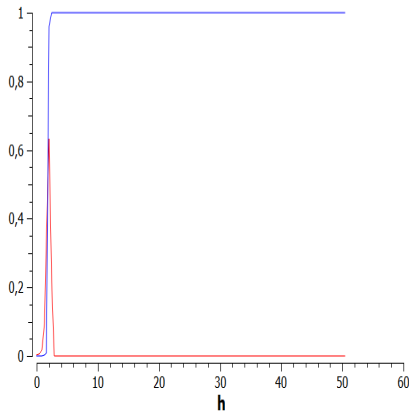
Figure 11.1: CDH1 and CDC20 in hyperactive-Ras cell treated with strong Raf inhibition or MEK inhibition.
