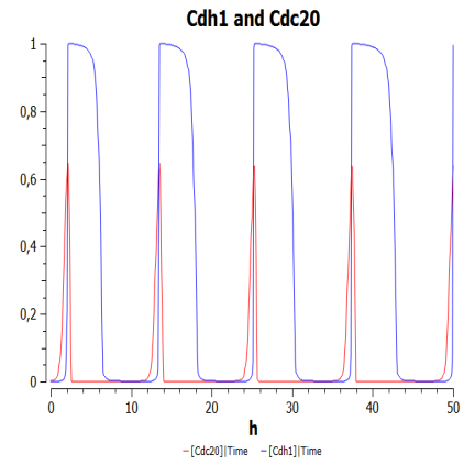
Figure 10.4: CDH1 and CDC20 in overexpressed-Cyclin D cell
