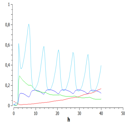
Figure 8.6: p27-CycA (red), p27-CycD 37 (dark blue), p27-CycE (green) and free p27 (light blue) with strong dependency on and fast production of GAP
