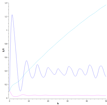
Figure 8.14: p21 (light blue), Hdm2 (dark blue) and p53 (pink) in CDH1 -deficient cell
