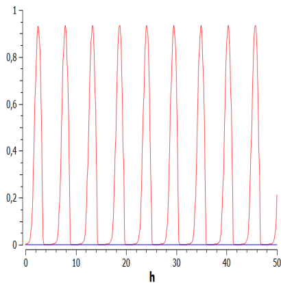
Figure 8.10: CDH1 (blue) and CDC20 (red) in CDH1-deficient cell
