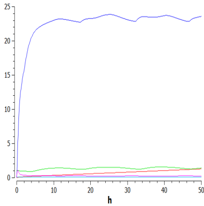
Figure 8.19: Hdm2 (dark blue), Caspase-9, p53 forms, p14 ARF and p21 in cell with mutated p53 such that it can no longer activate p21 synthesis
