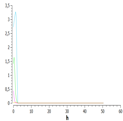
Figure 11.2: Cyclins concentration in hyperactive-Ras cell treated with strong Raf inhibition or MEK inhibition.
