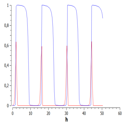
Figure 7.5: CDH1 (blue) and CDC20 (red) concentration
