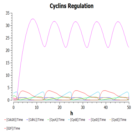
Figure 10.6: Cyclins regulation in overexpressed-Cyclin D cell
