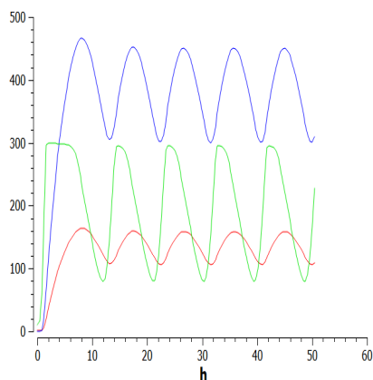
Figure 7.6: ERG (blue), DRG (red) and ERK (green) in healthy cell model
