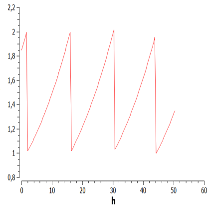
Figure 7.3: Mass of healthy cell model
