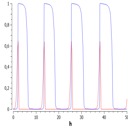
Figure 8.17: CDH1 (dark blue) and CDC20 (red) in Rb -mutated cell
