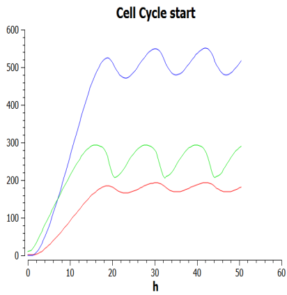
Figure 11.5: ERG (blue), DRG (red) and ERK (green) in hyperactive-Ras cell treated with ERK inhibition.
