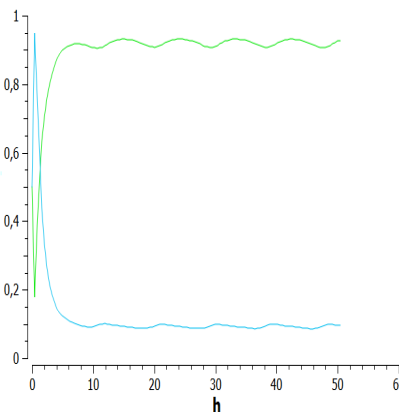
Figure 9.3: PIP3 (blue) and inactive PIP3:AKT (green) in hyperactive-AKT cell model
