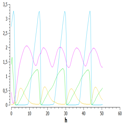
Figure 7.2: Cyclins A (green), B (blue), D (pink) and E (yellow) complexes concentration in healthy cell model
