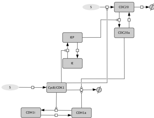
Figure 1.1: Reaction network. SBML representation in Cell Designer.
