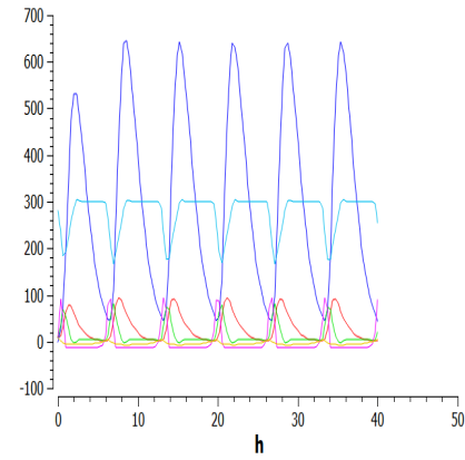
Figure 8.4: MAPK cascade components (red, green, pink, light blue, yellow) with strong dependency on and fast production of GAP (dark blue)
