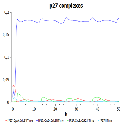
Figure 10.5: p27 complexes in overexpressed-Cyclin D cell
