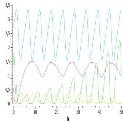
Figure 8.11: Cyclins A (green), B (light blue), D (pink) and E (yellow) in CDH1-deficient cell
