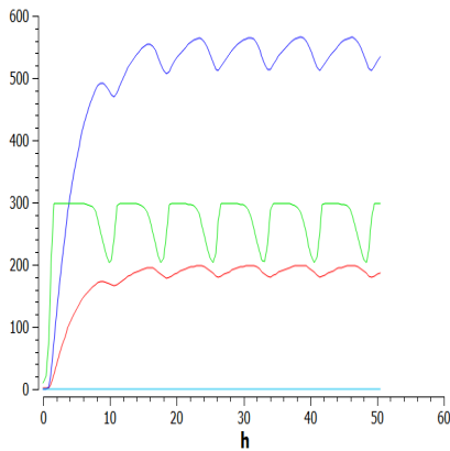
Figure 9.1: ERG (blue), DRG (red) and ERK (green) in hyperactive-Ras cell model
