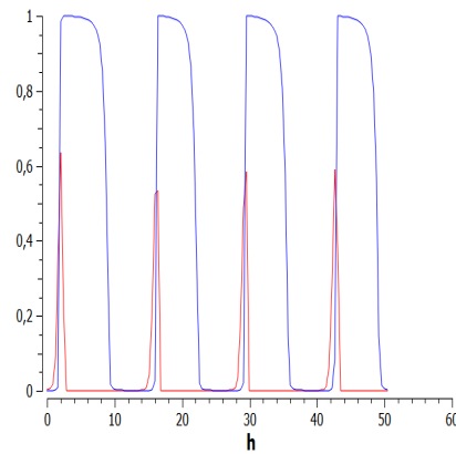
Figure 9.2: CDH1 (blue) and CDC20 (red) in hyperactive-Ras or hyperactive-AKT cell model
