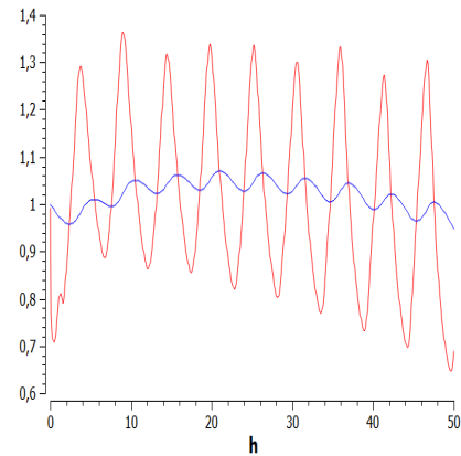
Figure 8.13: E2F and p14 ARF in CDH1 -deficient cell
