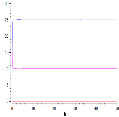
Figure 8.20: Hdm2 (dark blue), p53 (pink) and Caspase-9 (red) in cell with mutated p53 such that it can no longer activate Caspase9 synthesis
