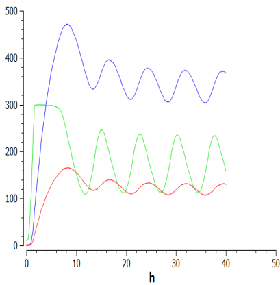
Figure 8.3: ERG (blue), DRG (red) and ERK-PP (green) with inefficient dephosphorylation of MEK-P
