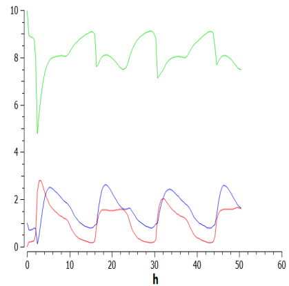
Figure 7.7: Hypophosphorylated Rb (green), active E2F (blue) and E2F:Rb complex (red) regulations in healthy cell model
