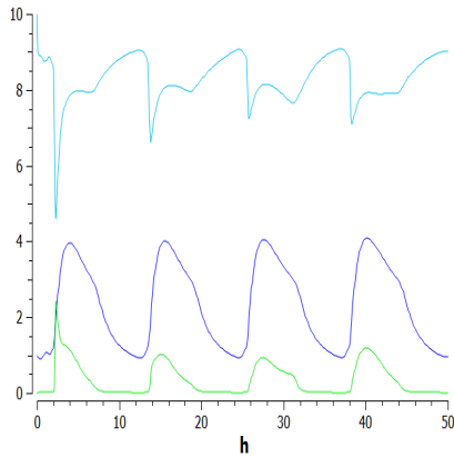
Figure 8.16: E2F (dark blue), active (light blue) and inactive (green) forms of Rb in Rb -mutated cell
