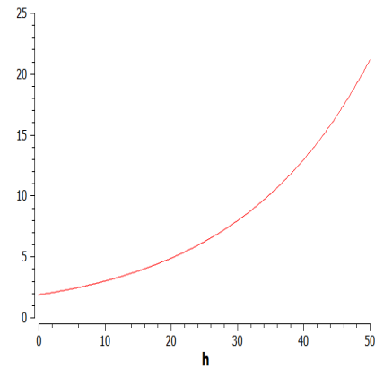
Figure 8.15: Mass in CDH1 -deficient cell
