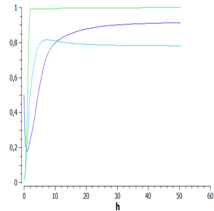
Figure 8.8: Active Rheb (dark blue), active (green) and inactive (light blue) mTORC1 in overactivated-PI3K cell model
