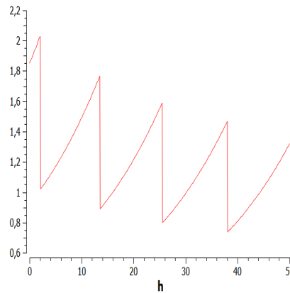
Figure 8.18: Mass in Rb -mutated cell
