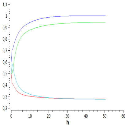
Figure 8.9: Active TSC1 (dark blue), active (light blue) and inactive (green) TSC2, and TSC1:TSC2 complex (red) in overactivated-PI3K cell model
