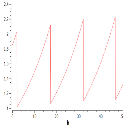
Figure 8.21: Mass in p53-mutated cell
