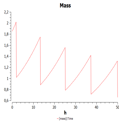
Figure 10.7: Mass in overexpressed-Cyclin D cell
