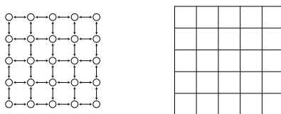
Figure 2. Two possible representations of the planar square lattice network with nearest neighbour coupling architecture.
