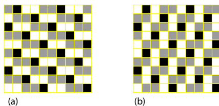
Figure 4. Two periodic colourings, each one is obtained from one decomposition of G_B into networks in Figure 3. For (a), the decomposition is based on \Gamma_1 = \langle\langle c_1c_2c_3c_4c_5 \rangle\rangle , with the permutation \sigma_1 = (c_1c_2c_3c_4c_5) associated with the horizontal direction and \sigma_2 = (c_1c_3c_5c_2c_4) with the vertical one. For (b), the decomposition is based on \Gamma_4 = \langle\langle c_1c_2c_4c_5c_3 \rangle\rangle , with the permutation \sigma_1 = (c_1c_2c_4c_5c_3) associated with the horizontal direction and \sigma_2 = (c_1c_4c_3c_2c_5) with the vertical one.
