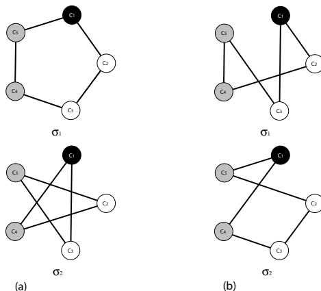
Figure 3. Two different decompositions of G_B into two networks with valence 2. To each one of the resulting networks we associate one permutation: for (a), \sigma_1 = (c_1c_2c_3c_4c_5) and \sigma_2 = (c_1c_3c_5c_2c_4) , both permutations belong to \Gamma_1 = \langle\langle c_1c_2c_3c_4c_5 \rangle\rangle ; for (b), \sigma_1 = (c_1c_2c_4c_5c_3) and \sigma_2 = (c_1c_4c_3c_2c_5) , both permutations belong to \Gamma_4 = \langle\langle c_1c_2c_4c_5c_3 \rangle\rangle .
